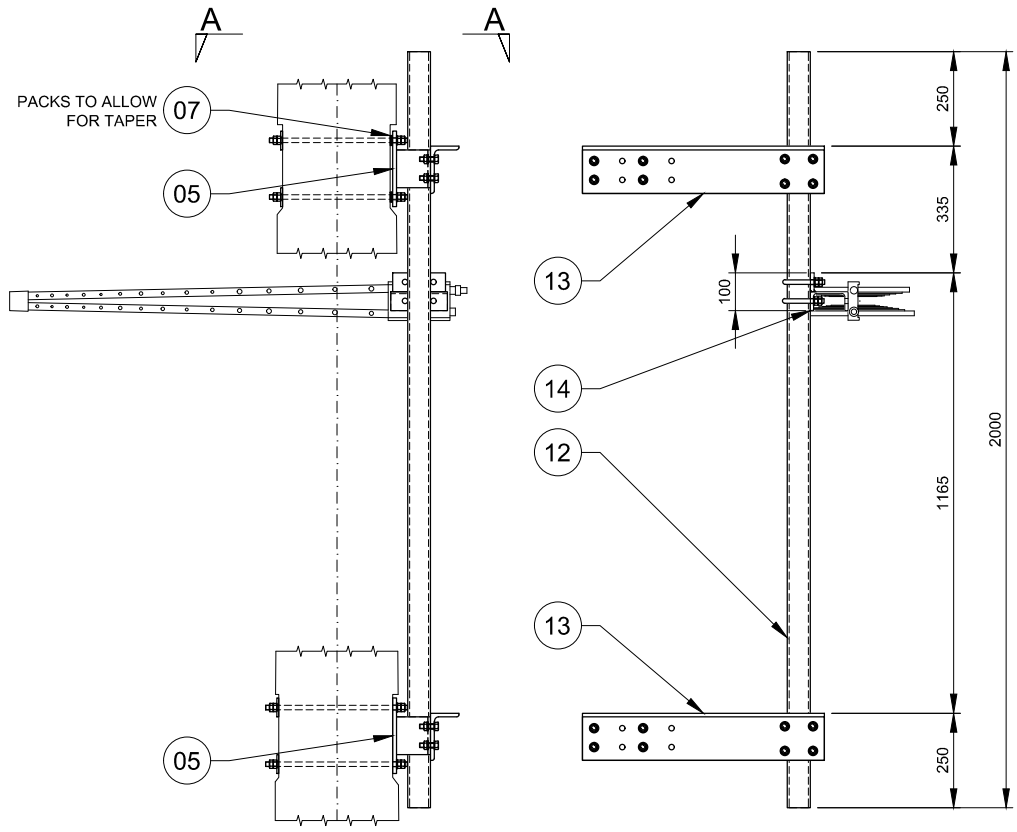
DETAIL H - Rx ANTENNA MOUNT Scale 1:20
