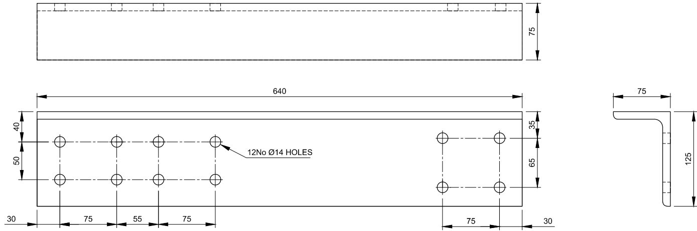
TPL-C - UA125x75x10 Scale 1:5
