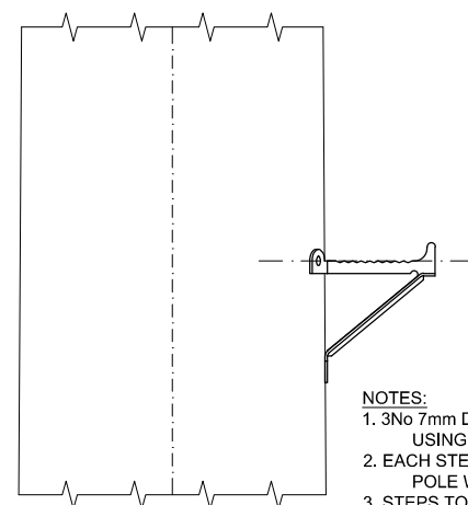
DETAIL D - ANTENNA ACCESS CLIMBING STEP Scale 1:10
