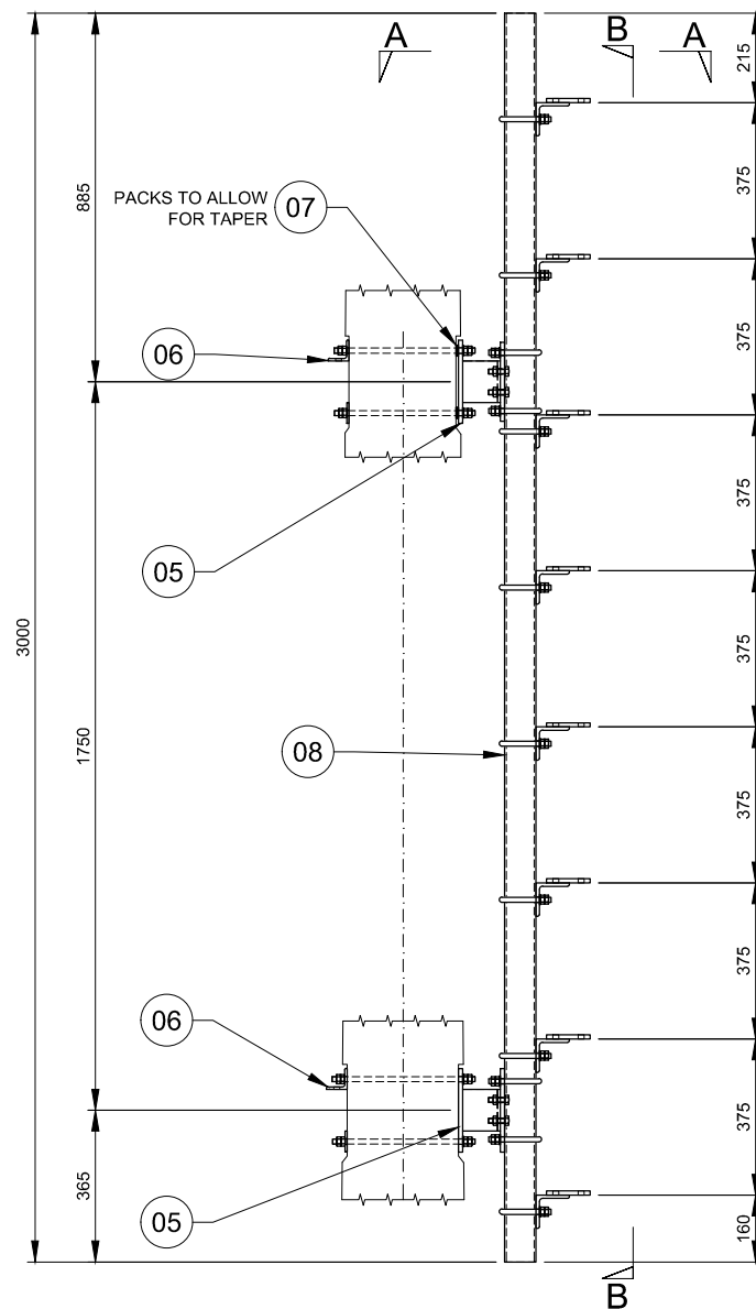
DETAIL G - Tx ANTENNA MOUNT Scale 1:20
