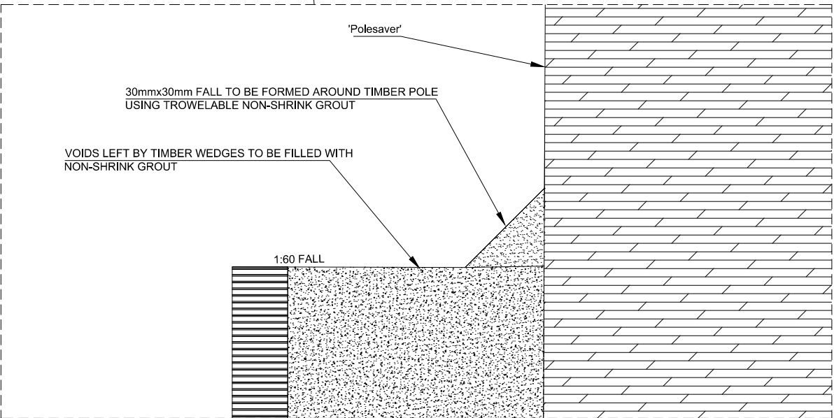
ENLARGED DETAIL Scale 1:2
