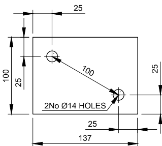
TPL-1 - 10mm THICK Scale 1:5
