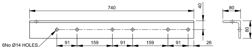
TPL-A-1 - EA 80x80x8 Scale 1:10
